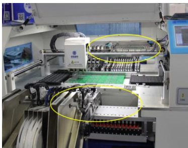
Double side 60pcs feeders
